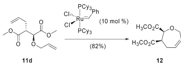
Scheme 4. RCM of diene 11d to oxepine 13 .
