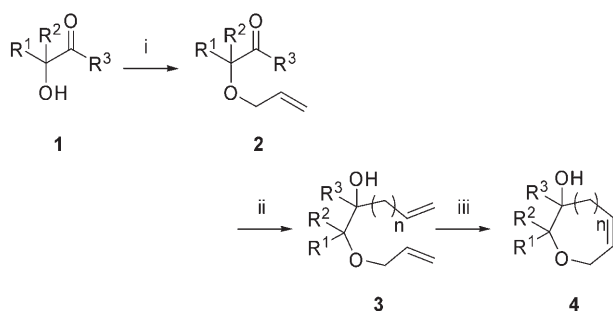
Scheme 1. Synthesis of functionalized oxacycles from \alpha -hydroxy carbonyl compounds based on olefin metathesis.
