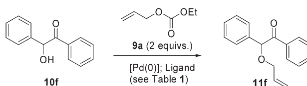
Scheme 3. Pd-catalyzed allylation of benzoin with allyl ethyl carbonate.
