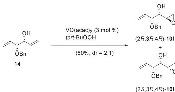
Scheme 6. V-catalyzed epoxidation of 14 .
