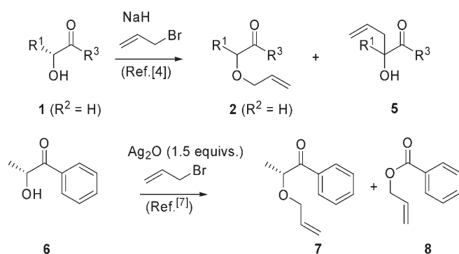
Scheme 2. Side reactions of established allylation procedures.
