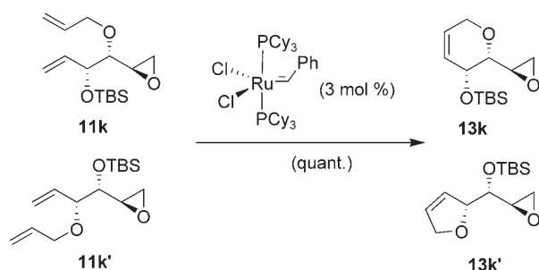
Scheme 5. RCM of the mixture of 11k and 11k' .
